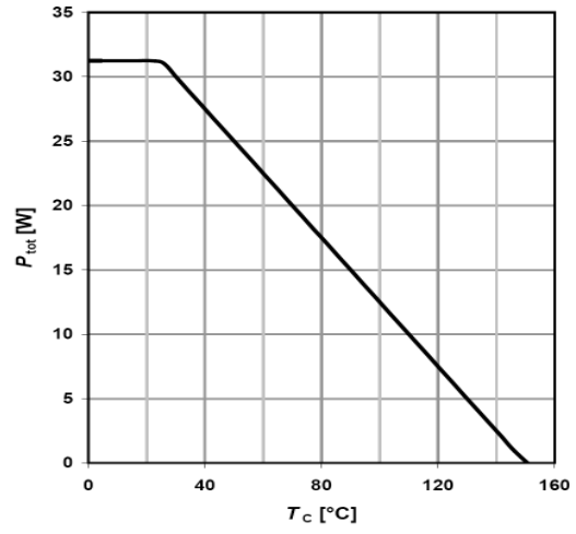
Figure 4: Power Dissipation
