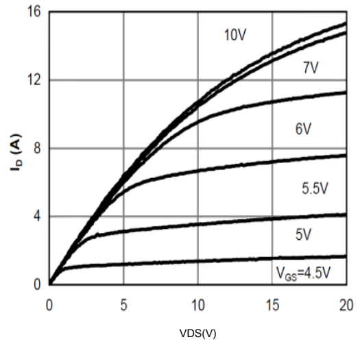
Figure 2: On-Region Characteristics@125°C
