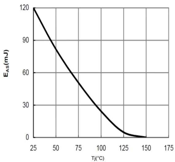
Figure 17: Avalanche energy
