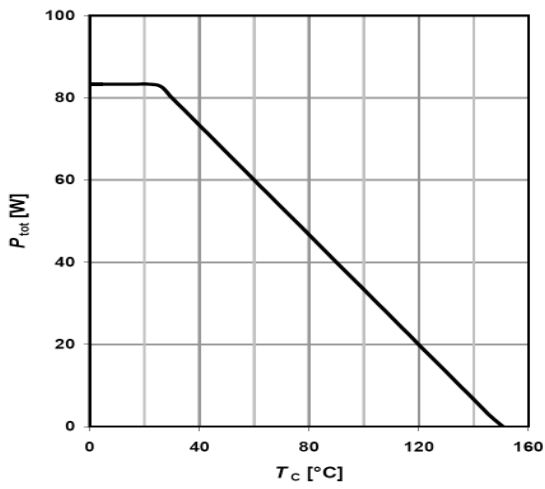
Figure 3: Power Dissipation
