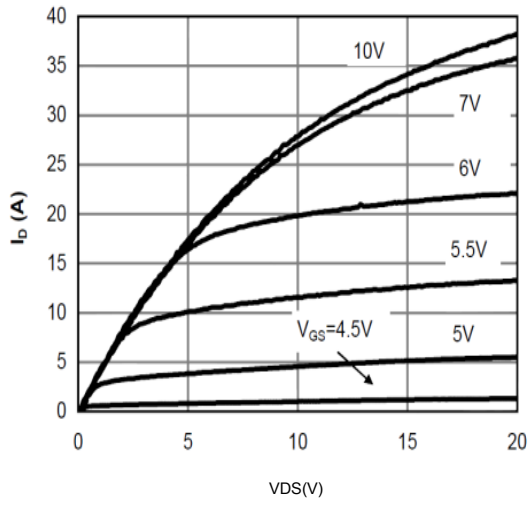
Figure 1: On-Region Characteristics@25°C
