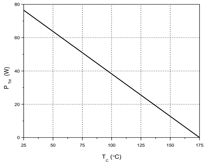
Figure 6. Power Derating
