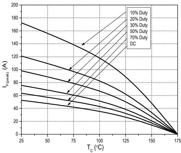
Figure 7. Current Derating
