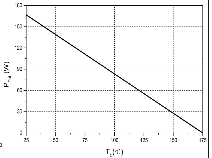
Figure 6. Power Derating
