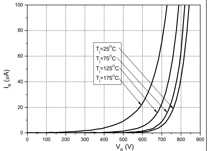
Figure 2. Reverse Characteristics
