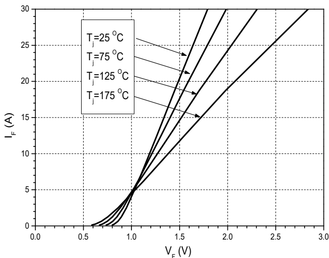
Figure 1. Forward Characteristics
