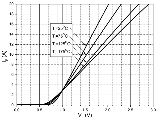
Figure 1. Forward Characteristics
