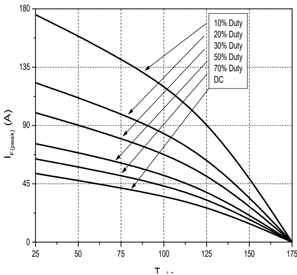
Figure 7. Current Derating
