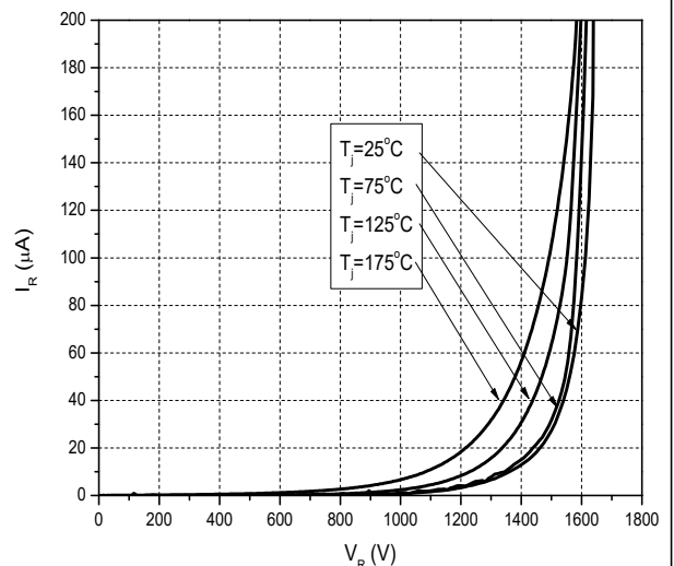
Figure 2. Reverse Characteristics
