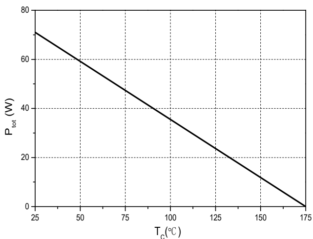
Figure 6. Power Derating
