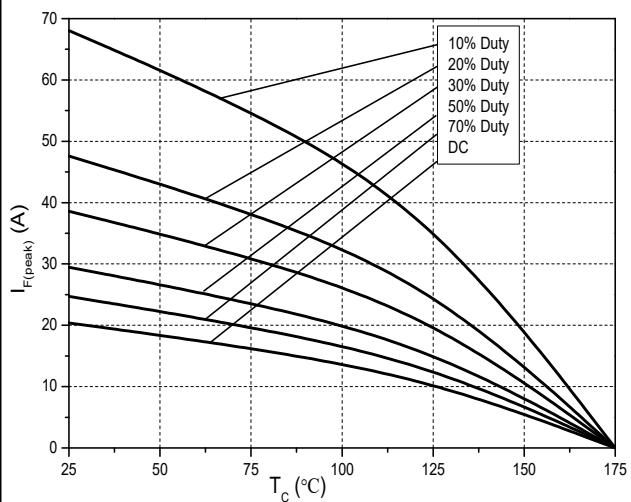
Figure 7. Current Derating
