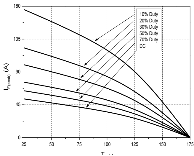
Figure 7. Current Derating
