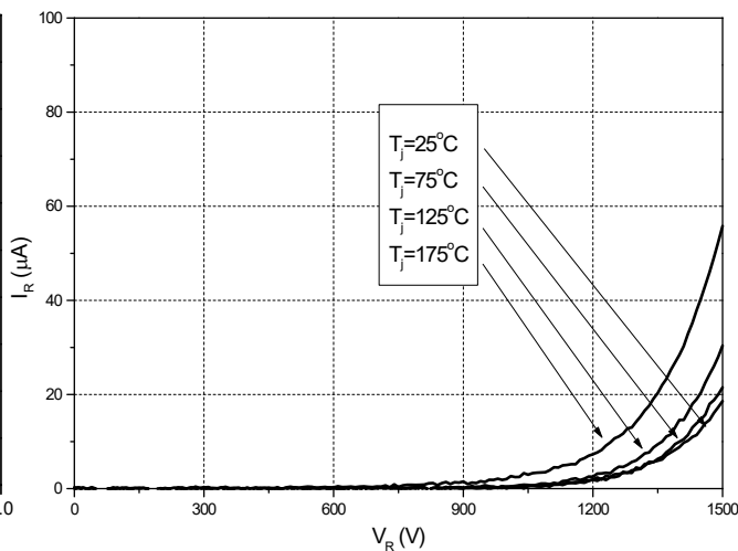
Figure 2. Reverse Characteristics
