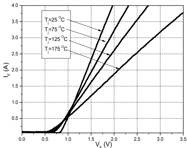
Figure 1. Forward Characteristics
