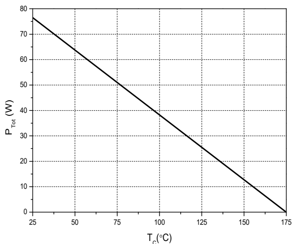
Figure 6. Power Derating
