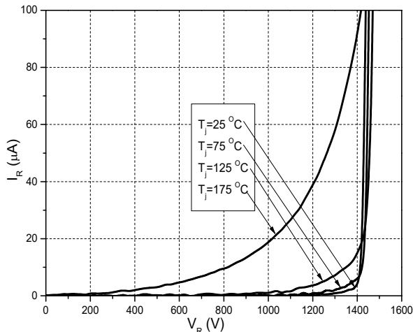
Figure 2. Reverse Characteristics
