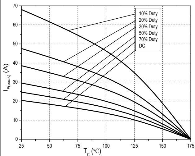
Figure 7. Current Derating
