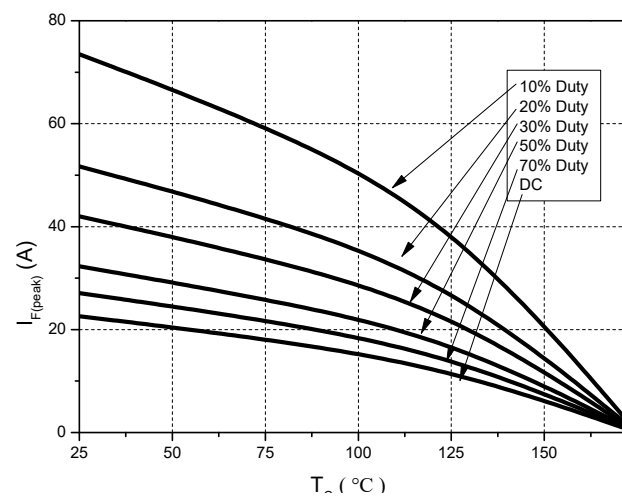
Figure 7. Current Derating
