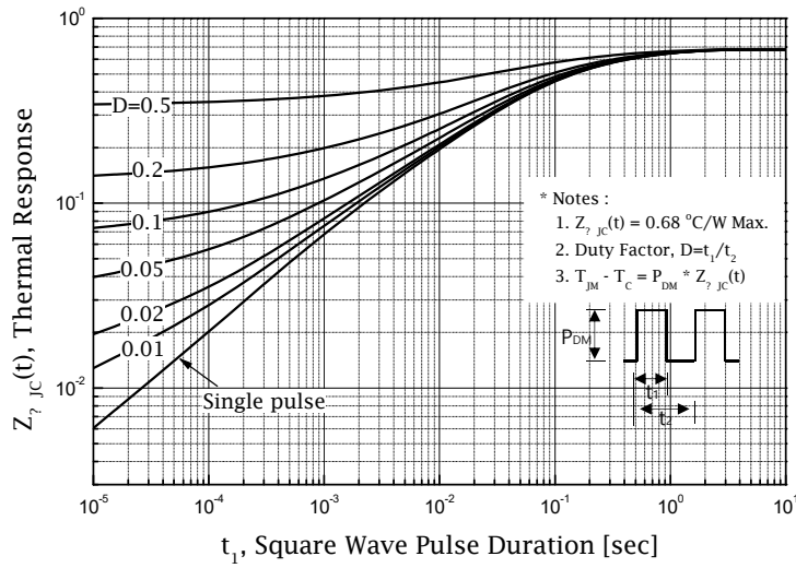
Figure 11-1. Transient Thermal Response Curve for SLP12N65S
