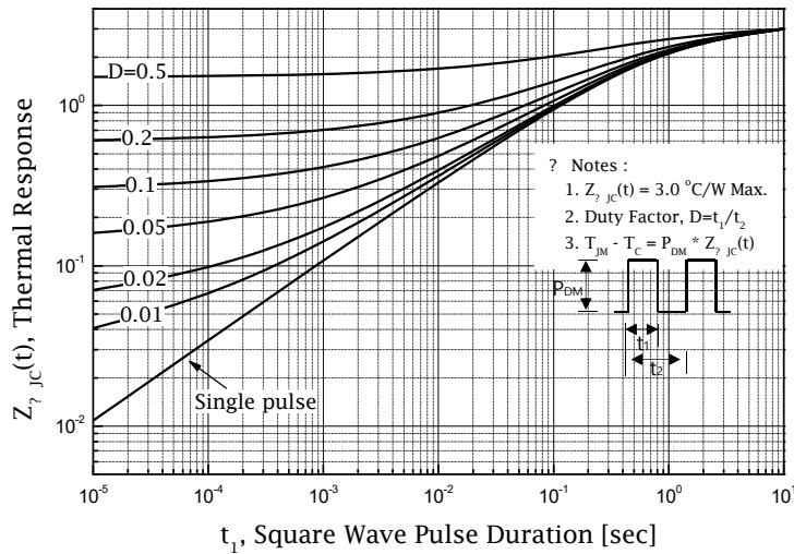
Figure 11-2. Transient Thermal Response Curve for SLF12N65S
