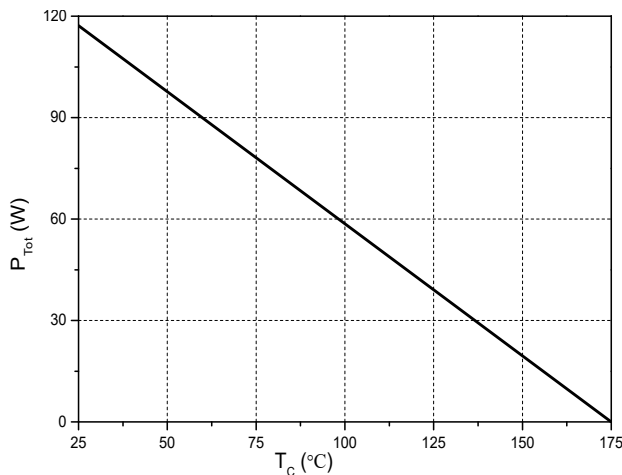
Figure 6. Power Derating
