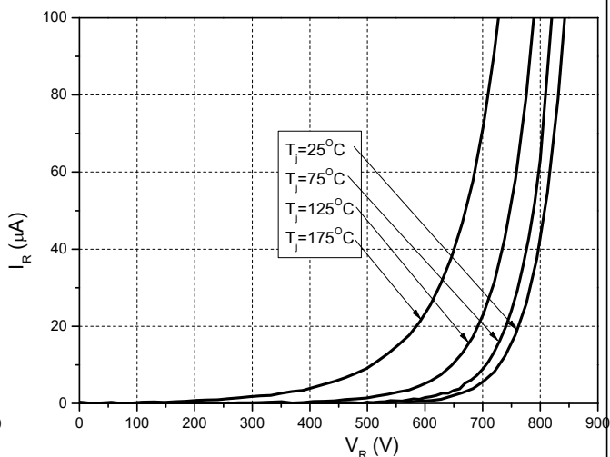
Figure 2. Reverse Characteristics
