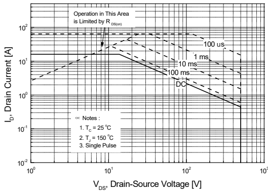
Figure 9. Maximum Safe Operating Area for SLB16N50C
