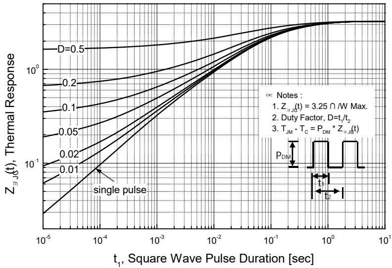
Figure 13-2. Transient Thermal Response Curve for SLF13N35UZ
