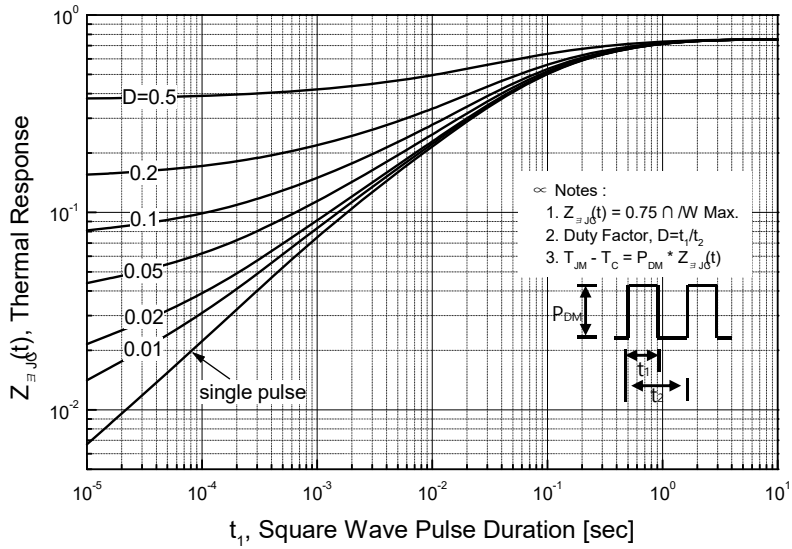
Figure 13-1. Transient Thermal Response Curve for SLP13N35UZ
