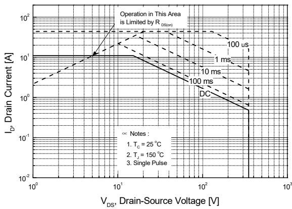
Figure 9-1. Maximum Safe Operating Area for SLP13N35UZ
