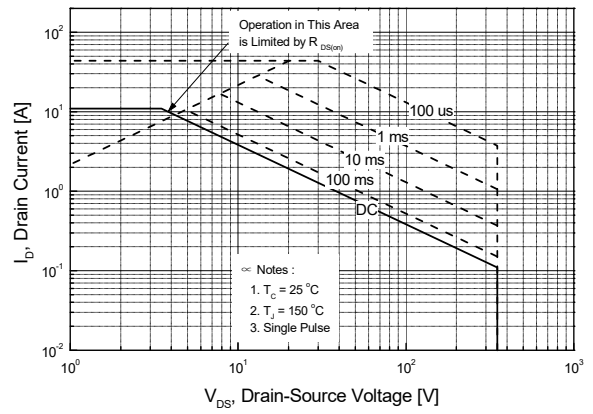
Figure 9-2. Maximum Safe Operating Area for SLF13N35UZ
